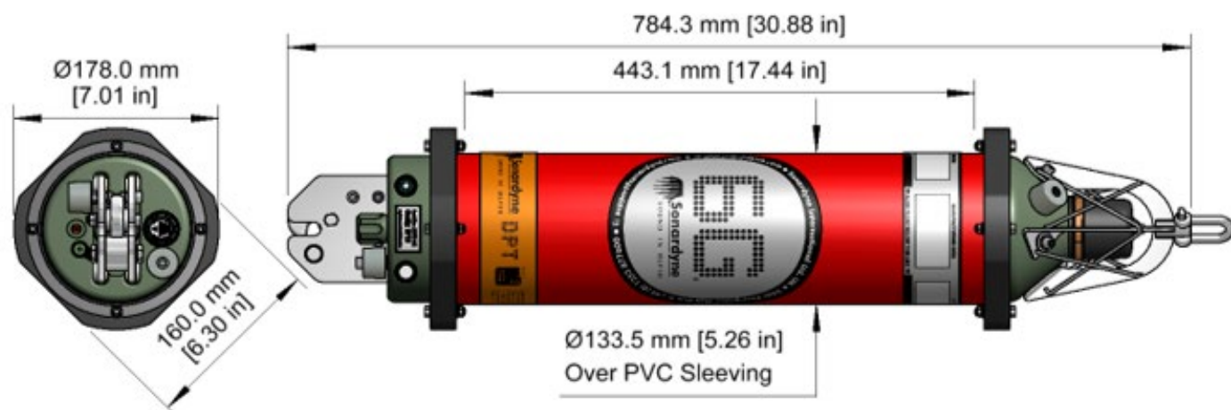
3 km Depth Rated MF Omni version shown (8301-3141)
